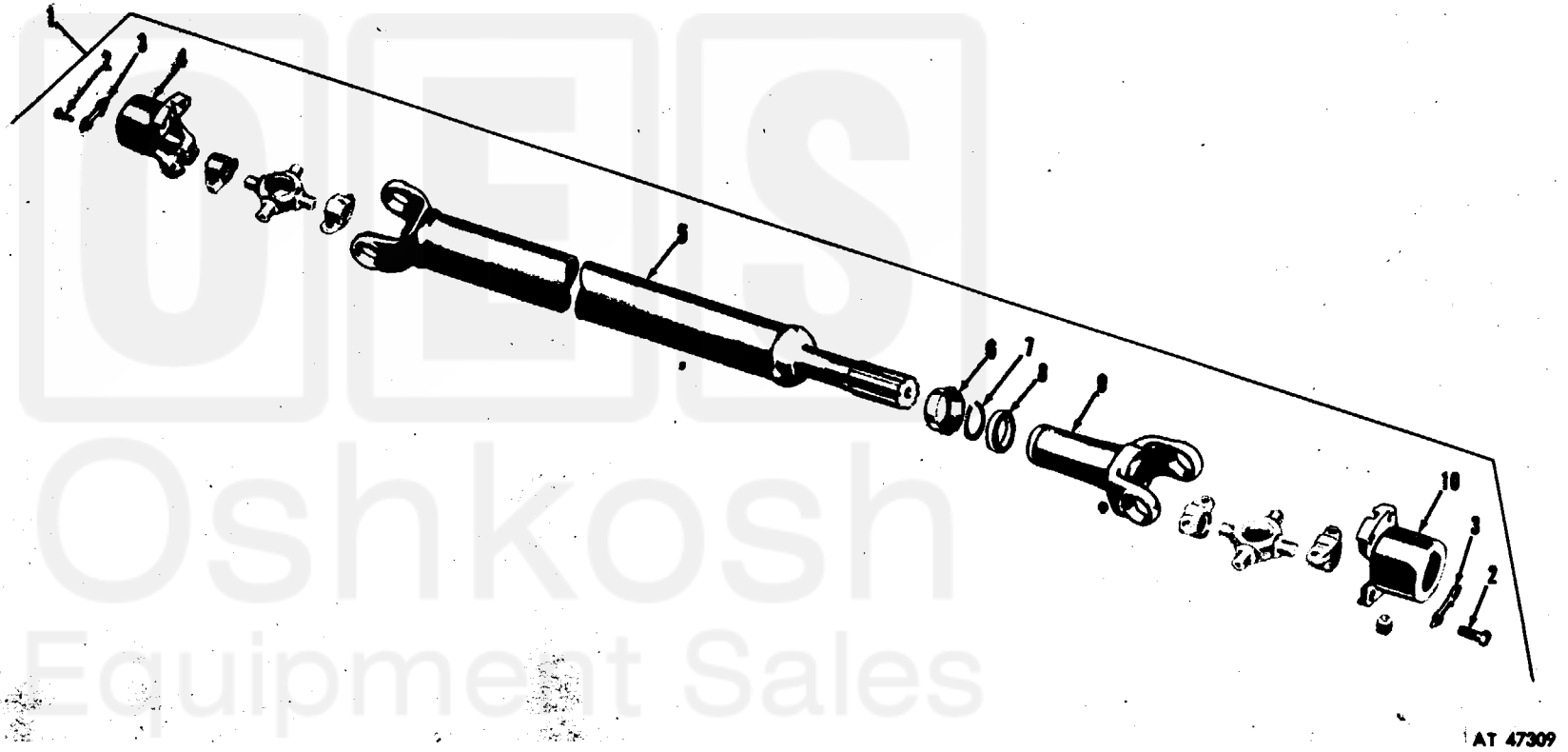
Figure 214. Front winch propeller shaft assembly.
